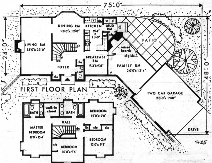
FLOORS PLANS: Spacious foyer leads directly to living room, kitchen, breakfast room and the second floor. Angled family room is accessible from the breakfast room, the patio and the two-car garage.
