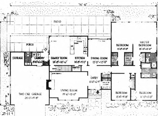
FLOOR PLANS: Complete separation of different areas of the house is emphasized in this interior pattern. Living area, garage are
