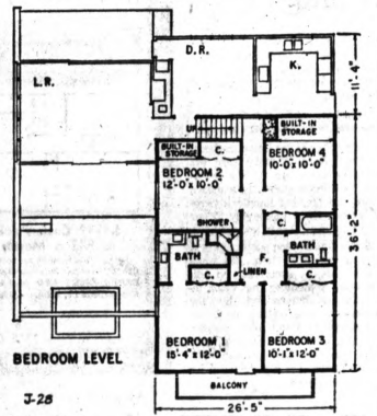
FLOOR PLANS —Only three steps divide formal and informal areas on lower levels, clearly separating them without excessive stair climbing. Upstairs foyer simplifies bedroom-level house-keeping. House contains 938 square feet on lower level; 938 square feet upstairs.
