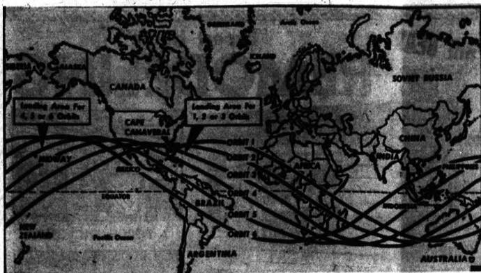
PLAN FOR ORBIT FLIGHT —The orbit paths and landing areas for a six-orbit U.S. space mission are plotted on this map based on a National Aeronautics and Space Administration release. Listed as a "three-plus orbit mission," the space trip is being planned for astronaut Walter M. Schirra for some time
