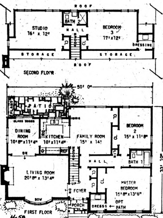
FLOOR PLANS: While maximum flexibility is the keynote of Design H-58, good traffic circulation is also apparent.
