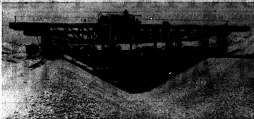
RED DITCH DIGGER — As tall as a four-story building and some 140 feet wide is this monster developed by the Russians for canal construction. It faces the sloping sides and bottom of a water channel and lays down a covering of concrete. It's powered by 16 electric motors.
