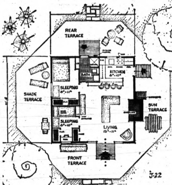
J-22 FLOOR PLAN — House is built on block piers, adaptable to any terrain; contains 576 square feet in dimensions of 24' by 24'. Note outside shower with adjacent entry from terrace to bathroom.
