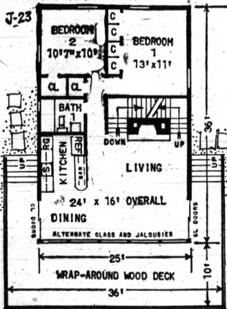
J-23 FLOOR PLAN — Basic house contains 900 square feet in dimensions of 25' by 36'; deck expands overall dimensions to 36' by 46'. Expansion balcony, to accommodate third bedroom and bath, would add 265 square feet of living area.
