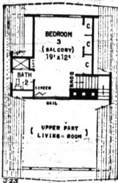
SHIP-SHAPE J-23: The profile of this 900-square-foot all-season home suggests the prow of a ship. Basically a two-bedroom house, it has a balcony expansion which would accommodate a third bedroom and bath. Overall dimensions are 36' by 46'.
