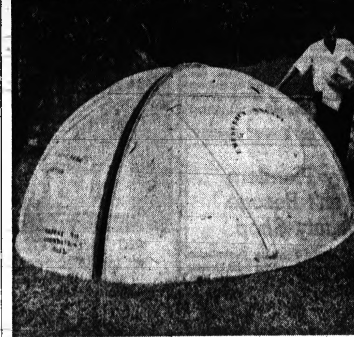
PLANS FOR SURVIVAL — Engineers for a shelter in Locust Valley, N.Y. The dome is designed to cover an excavation, being dug in the background, which is to be floored, walled and outfitted for emergency living.
