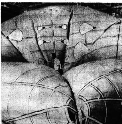
Partially inflated, like a giant pillow, the envelope bears markings showing where rudder and fins will be attached.
