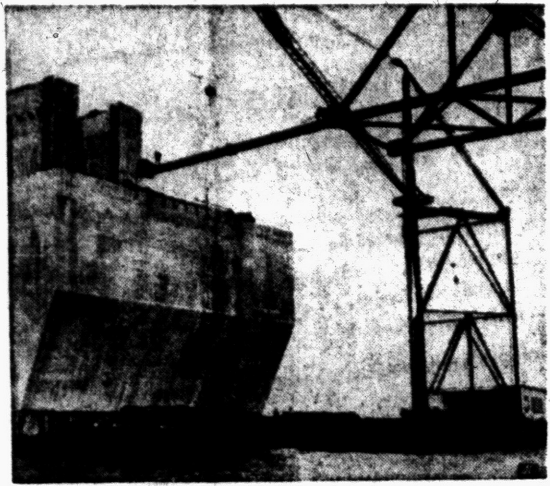
PENINSULAS LINKED — Workmen lower a steel beam into place on the Mackinac Bridge at Mackinac City, Mich., linking the upper and lower peninsulas of Michigan for the first time. The bridge spans the Straits of Mackinac and is scheduled to be completed next November.
