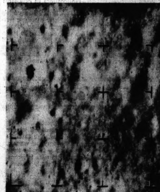
THREE MILES — Just 2.3 seconds before impact the view narrows down to area one and two-thirds miles in diameter. A crater at left near the top is about 300 feet in diameter. The smaller craters are about 30 feet in diameter.
