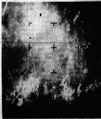
235 MILES — The historic flight of Ranger 7 gets a closer look at the lunar surface from 235 miles. The marks in the photo are to show any distortions due to the speed of the craft.
