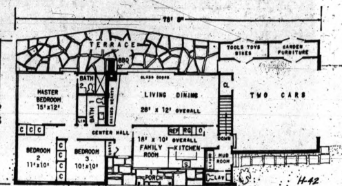
FLOOR PLANS — There's a complete separation of the living and sleeping portions of this house, with the indoor-outdoor living theme given a touch of privacy by Architect Lester Cohen's design.
