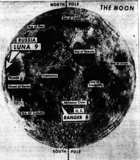
LANDING SPOT —This diagram shows the approximate area where Luna 9 accomplished a soft landing on the moon, according to an announcement today by the Soviet Union. The news agency Tass said the landing was in the area of the Ocean of Storms to the west of the crater Reiner.
