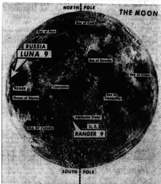
LANDING SPOT —This diagram shows the approximate area where Luna 9 accomplished a soft landing on the moon, according to an announcement today by the Soviet
