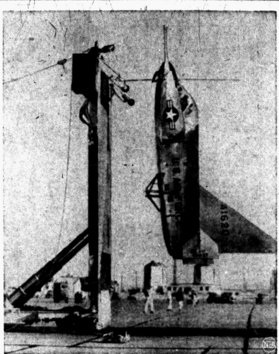
VERTIJET —The U. S. Air Force X-13 Vertijet, a jet-powered vertical take-off and landing research plane, takes off from a ground service trailer at Edwards Air Force Base, Calif. The plane, developed by the Ryan Aeronautical Co., made its first complete flight sequence last month. Rising and descending on a column of exhaust gases, the X-13 depends solely on thrust from its jet engine for both direct lift and level flight.
