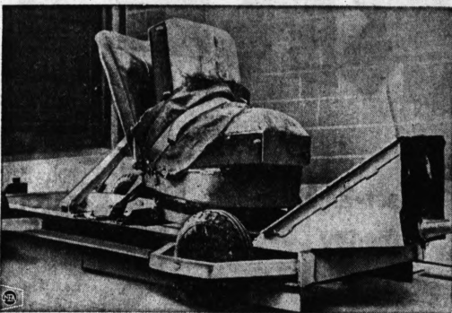
SWEDISH-DESIGNED — This sled was used in crash-simulation tests of auto seat belts by Consumers Union. Small cone at right is made of lead; it pancakes on impact to simulate the energy absorption of a car's front end in collision.
