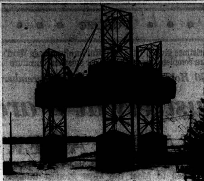
PORTABLE 'ISLAND' — Self-elevating platform, for use to reduce offshore oil drilling costs, dwarfs everything in sight on Mississippi River near Vicksburg, Miss. Platform, which stands on 140-foot legs, will be floated 400 miles downstream to Gulf of Mexico where it will be used as portable "island."
