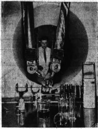
REMOTE CONTROL — These robot hands for handling radioactive materials were Czechoslovak displays at International Leipzig Spring Fair, East Germany.
