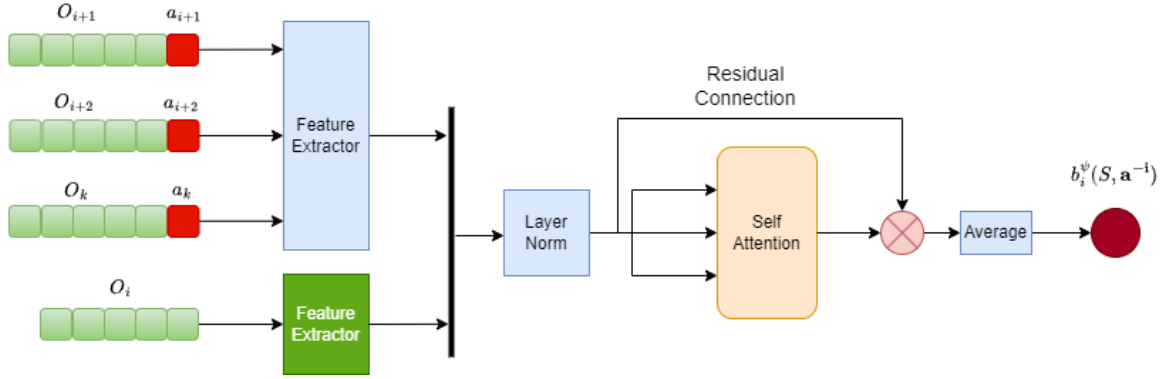
Figure 5.6: Baseline network architecture.
