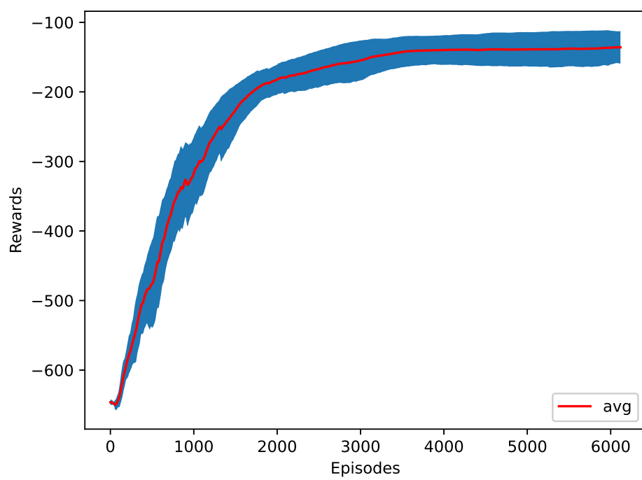
Figure 4.15: The training plot of the multi-objective reward function (Case 2).
