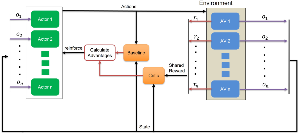
Figure 5.3: CTDE Actor-Critic MARL Architecture adopted in the proposed merging control framework.
