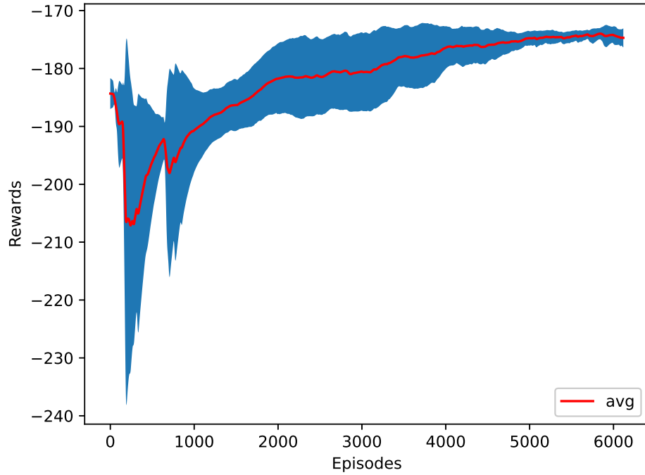
Figure 4.10: The training plot of the time as a reward function.
