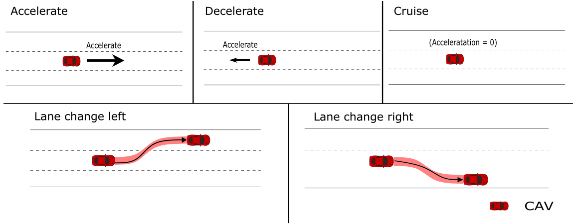
Figure 3.3: High level action space.
