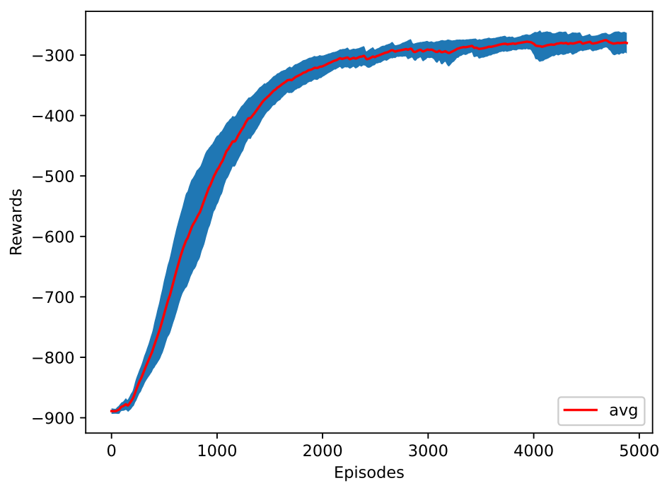
Figure 4.9: The training plot of the energy as a reward function.
