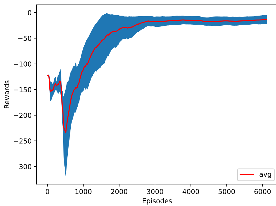
Figure 4.14: The training plot of the multi-objective reward function (Case 1).
