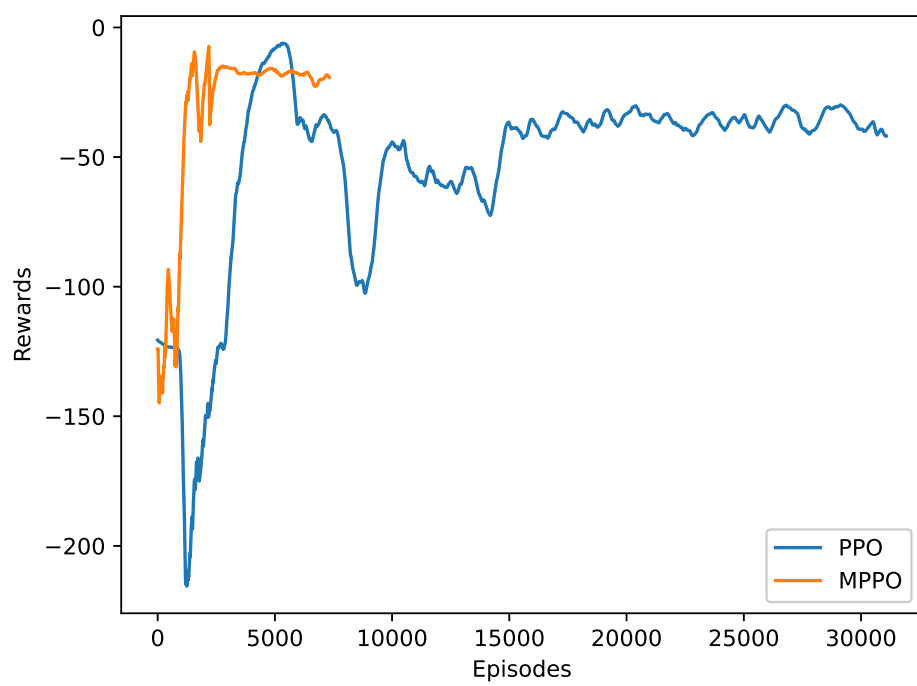
Figure 4.8: Comparison of training progress of MPPO and PPO.
