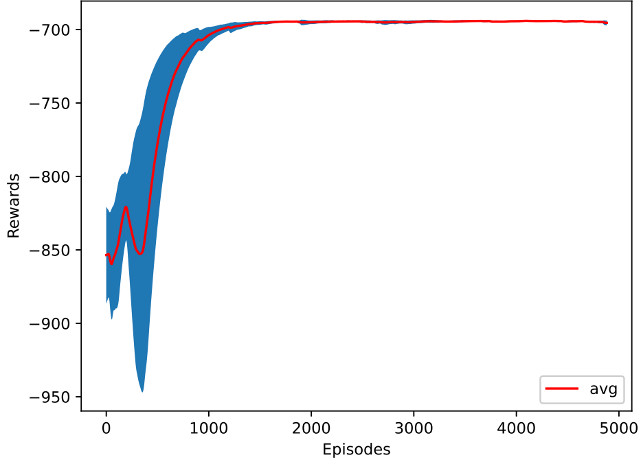
Figure 4.13: The training plot of the maximum jerk as a reward function.
