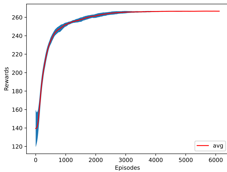
Figure 4.11: The training plot of the speed as a reward function.
