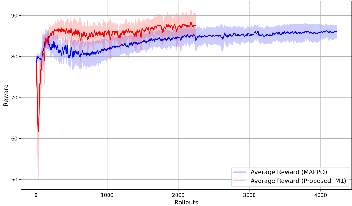
Figure 5.7: Convergence comparison of the proposed method (M1) and the benchmark MAPPO method.
