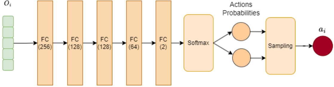
Figure 5.4: Actor network architecture.
