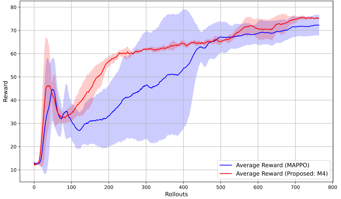
Figure 5.10: Convergence comparison of the proposed method (M4) and the benchmark MAPPO method.
