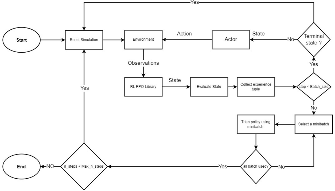
Figure 4.5: Data flow diagram of the PPO algorithm.
