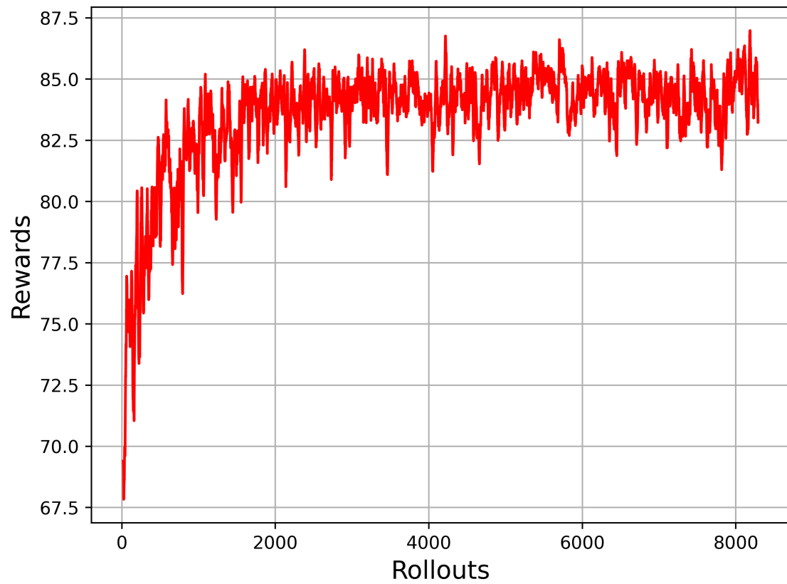
Figure 6.1: Learning curve for R1 reward function.
