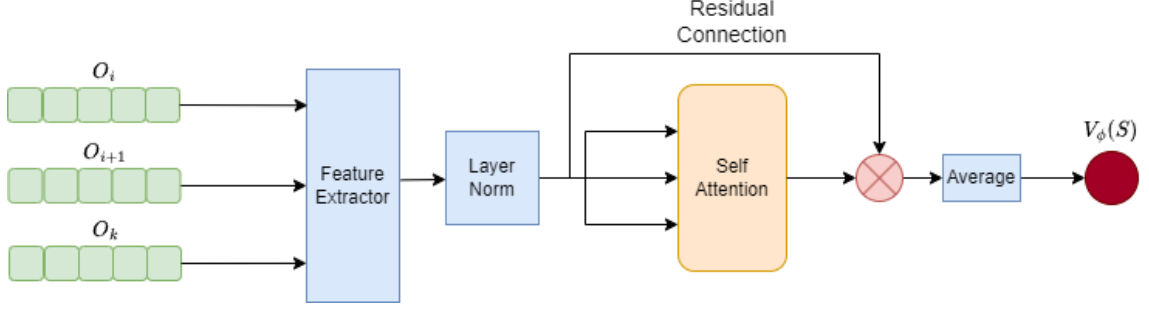
Figure 5.5: Critic network architecture.
