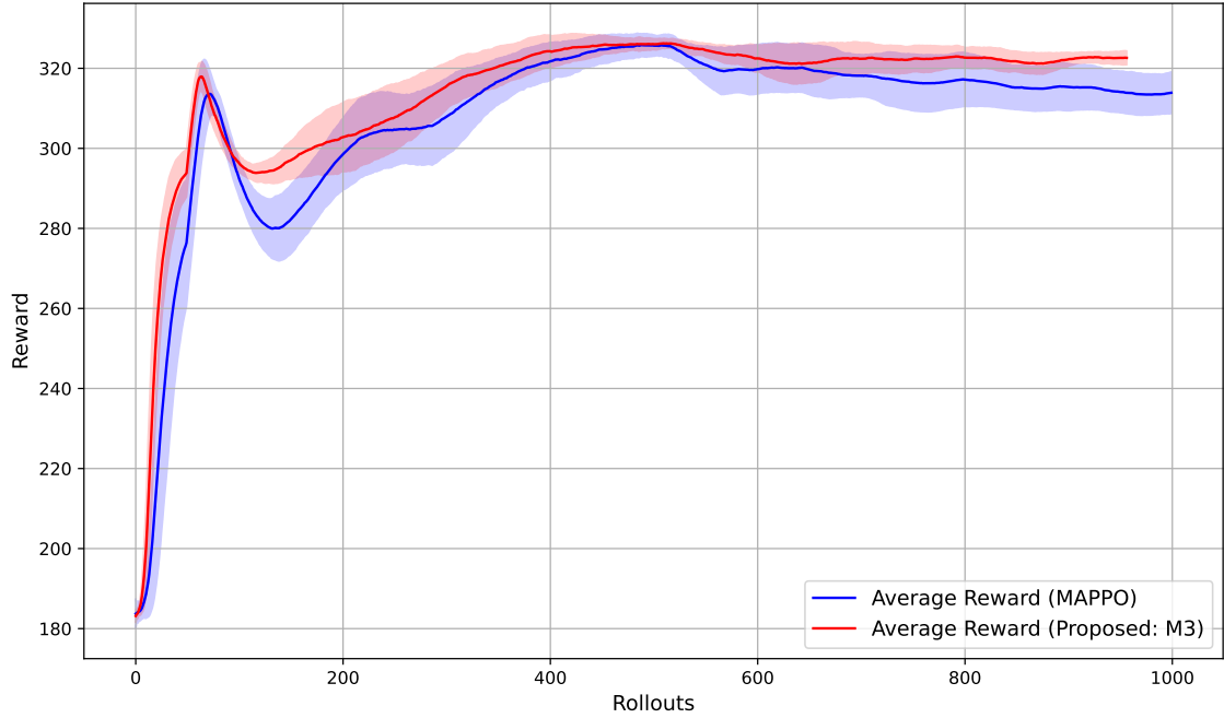
Figure 5.9: Convergence comparison of the proposed method (M3) and the benchmark MAPPO method.
