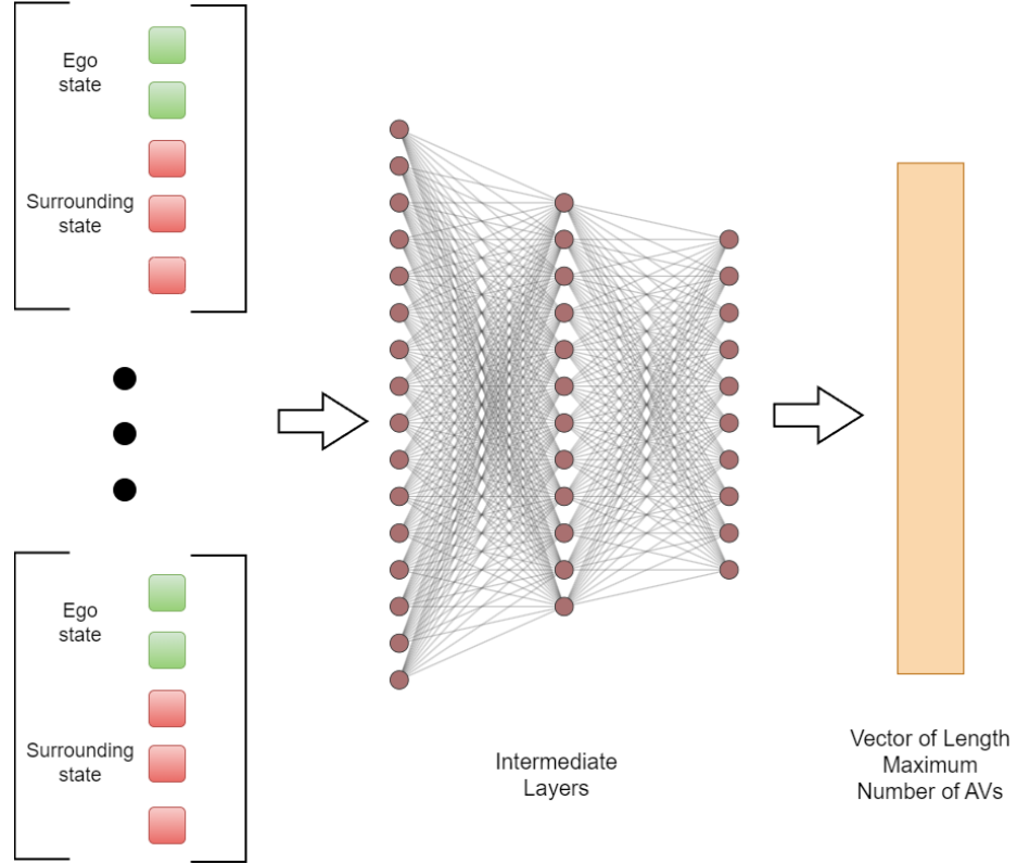
Figure 2.1: CTCE RL: Centralized policy processes all vehicles' observations and outputs all vehicles' actions. The input block is repeated by n times, where n is the maximum number of AVs, and the output is a vector of the length same as the maximum number of AVs.
