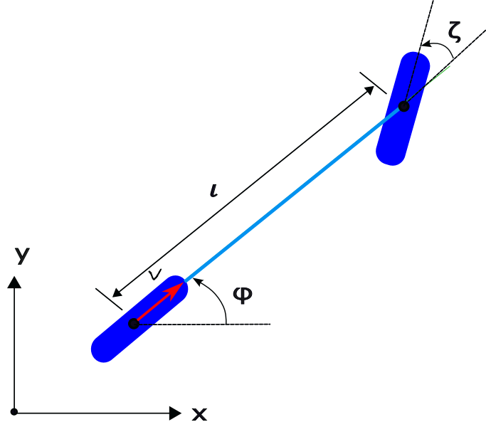
Figure 4.3: Schematics of the vehicle dynamics model.
