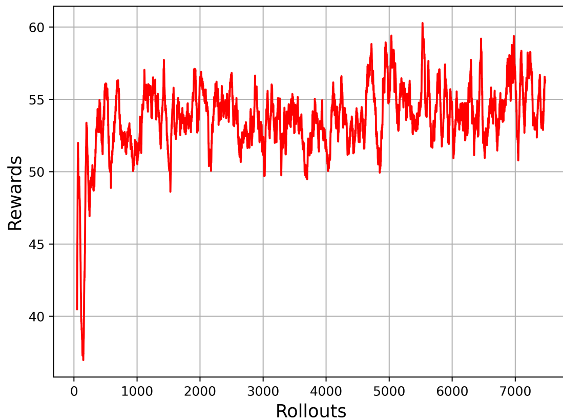
Figure 6.3: Learning curve for R3 reward function.
