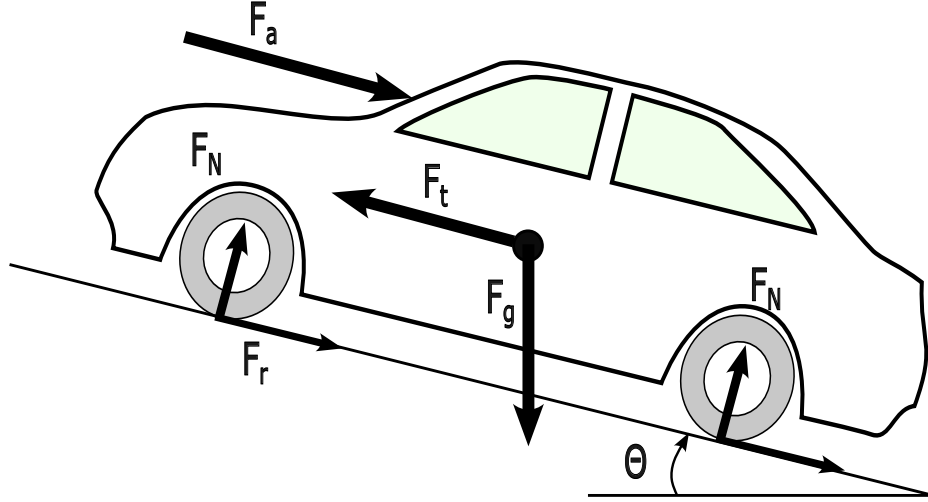
Figure 4.7: Free Body Diagram of the vehicle.
