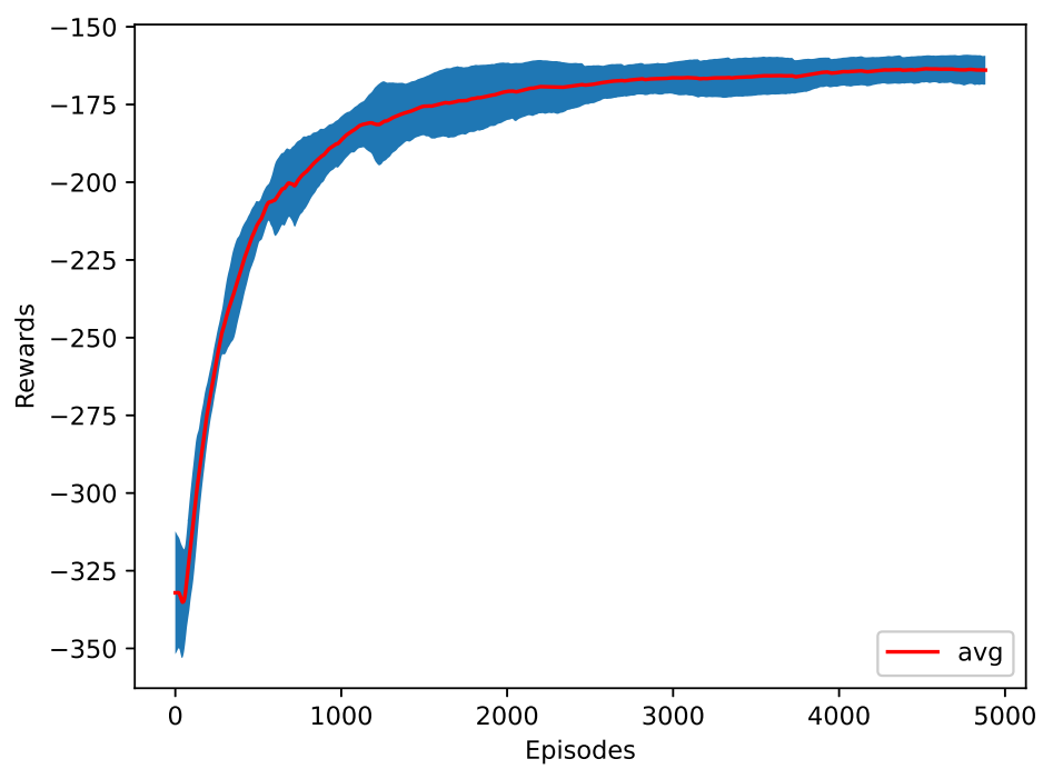
Figure 4.12: The training plot of the average jerk as a reward function.
