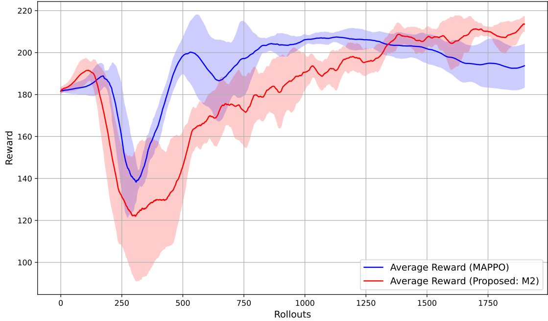
Figure 5.8: Convergence comparison of the proposed method (M2) and the benchmark MAPPO method.
