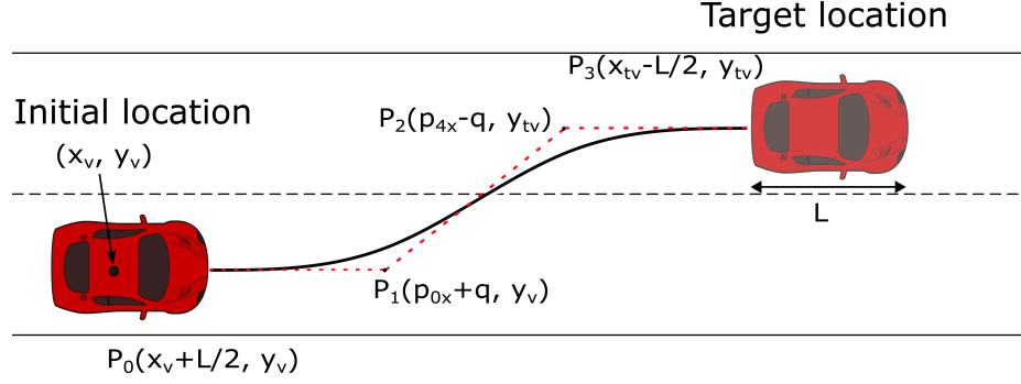
Figure 4.4: Lane changing cubic Bézier curve.
