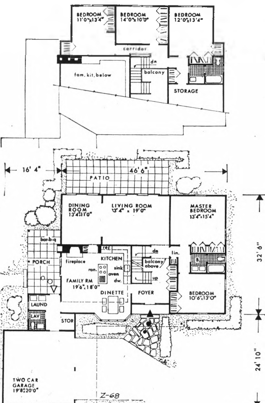
FLOOR PLANS: Lower floor shows excellent layout for family requiring only two bedrooms, with informal and formal sections clearly delineated and with side and rear outdoor living areas. Large families can utilize all or part of second floor for extra bedrooms.
