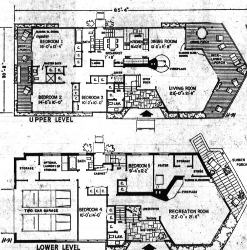
FLOOR PLANS: Two-level plan permits all main rooms to be located on upper floor, with huge areas for outdoor living; extra rooms, including fireplace recreation section and two-car garage, are on the lower floor.
