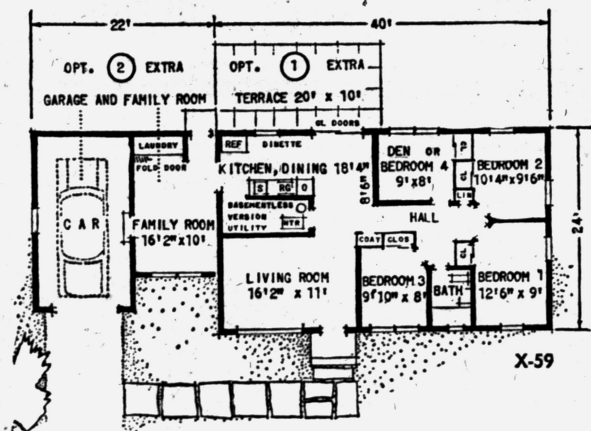
FLOOR PLAN — Note how the bedroom hall expands into an interior foyer, preventing a feeling of congestion in the sleeping section. The house can be constructed either with or without a basement. The family room and garage also are optional.
