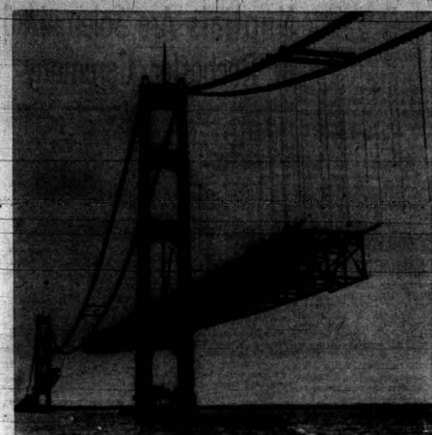
BRIDGE ROADWAY TAKES SHAPE — Now more than 60 per cent finished, the steel trusses that will support the roadway for the Mackinac Bridge suspended from cables attached to the main cables of the structure. This phase of the work is expected to be finished by the end of this month. The bridge, the world's largest suspension structure, is scheduled to be open to traffic on or about Nov. 1.
