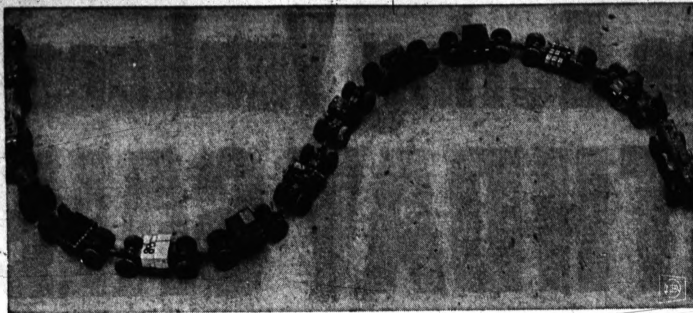
IT GOES 48-HUMMMM—Electric motors—one for each of its 54 giant-tired wheels—powers this experimental Overland Train, snaking its way across the sands at the Army's Yuma Test Station, Yuma, Ariz. Cab (far right) houses crew of six.
