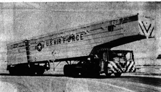
GIANT MISSILE CARRIER —Produced by GMC Truck & Coach Division, the Minuteman ICBM transporter-erector (shown above) is the largest vehicle ever produced for use on
