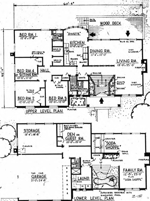
FLOOR PLANS — Plenty of space here for good living by a large family, with five possible bedrooms, a living room 25' long, a family room the same length, an outdoor wood deck accessible from the living room and kitchen, and lots of storage and closet areas.
