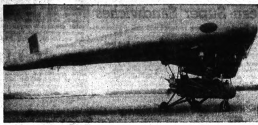
AIR ON THE WING —The "Flying Li-Lo" an inflated-wing aircraft, is checked out at Andover, England. The simple, open-cockpit fuselage is hung beneath the rubberized fabric wing. Deflated, the wing is easily packed and transported for military and observation flights.
