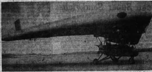
AIR ON THE WING — The "Flying Lo-Lo," an inflated-wing aircraft, is checked out at Andover, England. The simple, open-cockpit fuselage is hung beneath the rubberized fabric wing. Deflated, the wing is easily packed and transported for military and observation flights.
