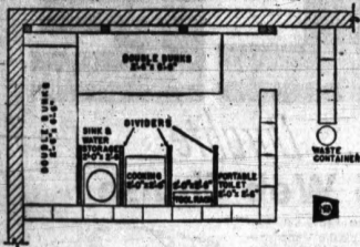
LAYOUT — This is the floor plan of basement fallout shelters. Details on construction may be obtained from your nearest civil defense headquarters or from the federal office at Battle Creek, Mich.
