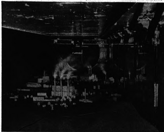
Industrial complex scale model testing in wind tunnel.
