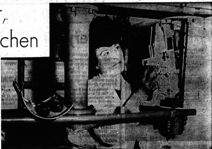
Mrs. Barbara Gordon of Birmingham illustrates how the electrically programmed holder (which usually contains a monkey) is placed inside the Mark I Space Flight Acceleration Profile Simulator (SFAPS) machine. Changes in the cardiac activity, brain wave currents, temperature and respiration of the animal caused by the acceleration experiment, are observed and reported.
