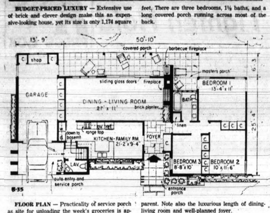
Brick Ranch Home Offers Excellent Floor Plan FLOOR PLAN—Practicality of service porch as site for unloading the week's groceries is apparent. Note also the luxurious length of dining-living room and well-planned foyer.
