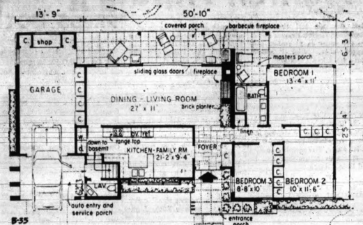
FLOOR PLAN — Practicality of service porch as site for unloading the week's groceries is apparent. Note also the luxurious length of dining-living room and well-planned foyer.
