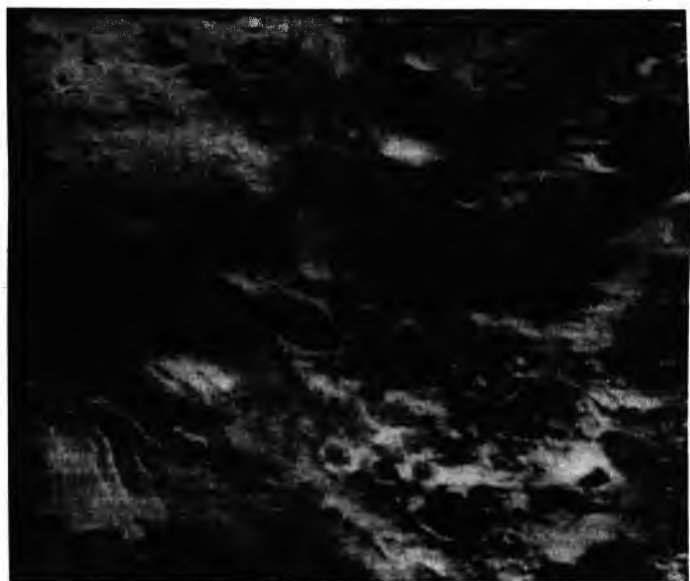
'LIKE BABY PICTURE OF EARTH' — This wide-angle view of Mars made by Mariner 7 from a distance of about 3,600 miles shows a variety of craters plus some distinct hills at lower left. "We may be looking at baby pictures of earth,"
