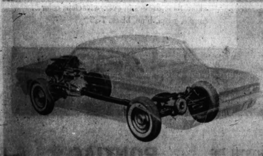
TRANSMISSION PLACEMENT — Rear location of the transmission in the new Tempest is shown in the picture above with the new four-cylinder engine up front. All four wheels are independently suspended, which provides exceptional handling and comfort. Three axle ratios are available: standard, 3.55:1; economy, 3.31:1; and performance, 3.73:1.
