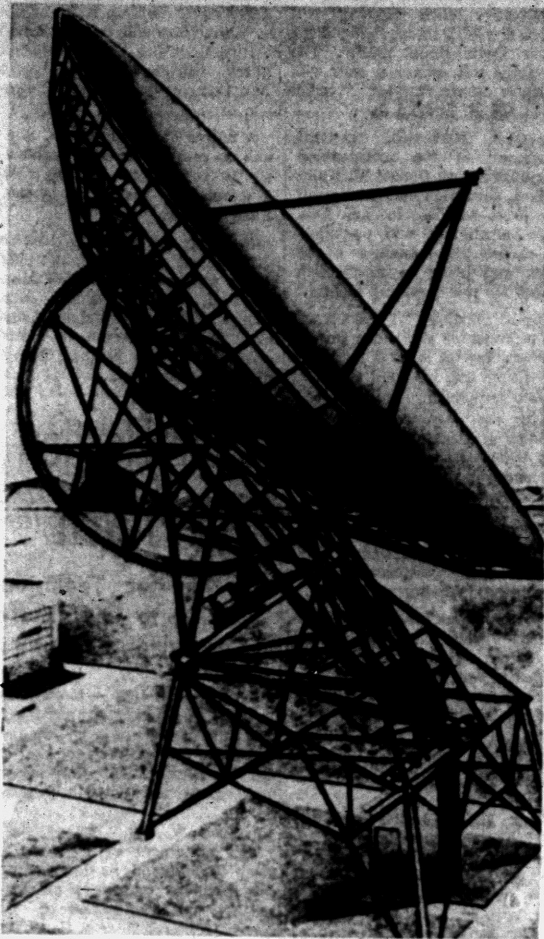
GIANT EAR FOR U. OF M. — This is a drawing of the huge radio telescope to be constructed near Ann Arbor next June for University of Michigan astronomers. The giant ear, 85 feet in diameter, will "listen in" on celestial objects ranging from such nearby bodies as the moon and sun to galaxies hundreds of millions of light years distant. It will be the second largest steerable radio telescope in the world. The largest is 250 feet wide, located at the University of Manchester in England.
