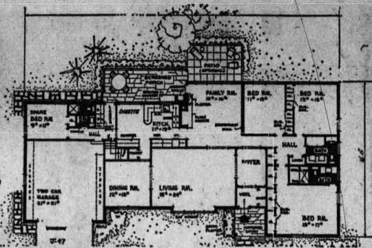
FLOOR PLAN —The house contains 2,504 square feet of living area not counting the 231-square-foot garage, in dimensions of 88'2" wide by 41' deep. Note the uncommon amount of closet and storage area, and the use of closets to soundproof the bedroom wing. House has a full basement.
