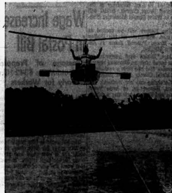
"BOATCOPTER"—Trying a new version of the "Look Ma, no hands" routine, aircraft designer Igor Bensen shows off his new helicopter boat at Gresham Lake, near Raleigh, N. C. Bensen says the rotor-lifted craft towed by a motorboat, is as easy to handle as a bicycle. Bensen heads the company bearing his name at Raleigh-Durham Airport, which is engaged in manufacturing one-man helicopters.
