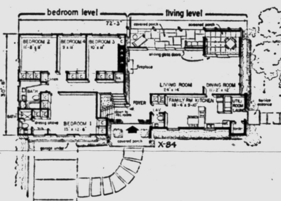
UPPER LEVELS—Diagram of bedroom and living level shows generous size of rooms. Area of these two sections is 1,926 sq. ft.
