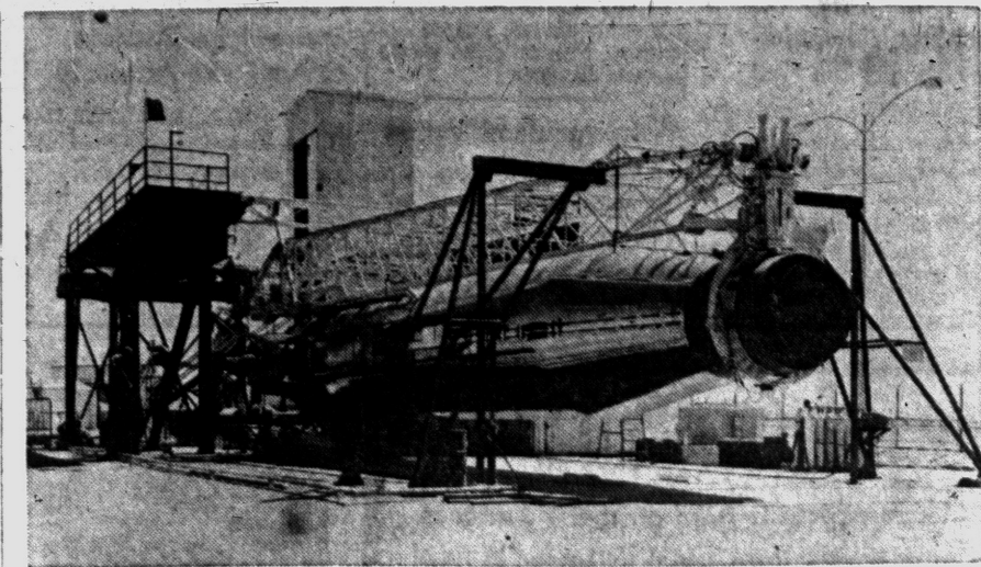
SIMPLE RIG LAUNCHES ATLAS — A new simplified launching system for the Atlas ICBM has been developed to eliminate huge gantry crane usually employed. The missile is stored horizontally, below, clamped by the nose on a 70-foot erector boom. In less than two minutes, fueled and fired, right. Clamp released the fuel led and fired, right. Clamp released, the boom is taken away. The 100-ton Atlas is lifted into this position by a 75-horsepower electric motor. First new installation will be made at Warren Air Force Base, Wyo.
