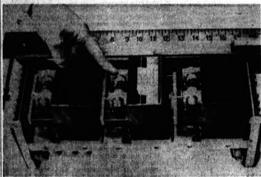
TINY BUT POWERFUL — The hand is pointing at a tiny relay device of the Ontario Hydro Electric Power Commission like the one which failed last Tuesday and blacked-out the northeast portion of the U.S. in the process. Breakdown of the relay in Hydro's Sir Adam Beck No. 2 generating station at
