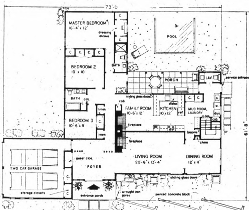
FLOOR PLANS: Practical traffic pattern permits movement from the oversized foyer directly to the living room-dining area, the family room-kitchen combination or the bedroom wing. Circulation layout is further enhanced by the multiplicity of entrances to house.
