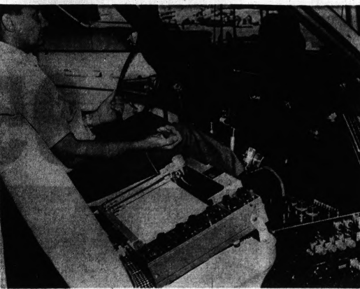
BRAKE DATA — A new machine to improve the quality of automobile brake testing is shown in operation at General Motors Proving Ground in Milford. Electronically controlled, it supplants the driver's foot and insures a much higher degree of test repeatability than human test drivers could provide.
