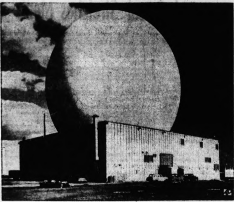
GIANT SPHERE PROTECTS RADAR — System (BMEWS). High-powered transmitting apparatus and complex computers in the base building are designed to detect and track missiles 2,000 miles away.
