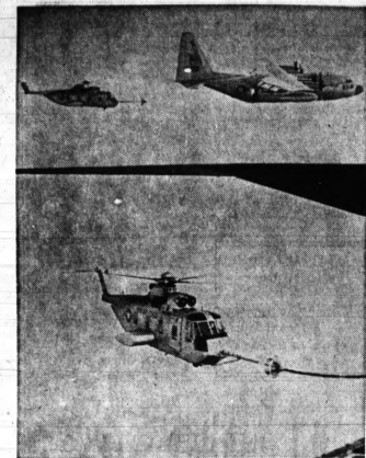
REFUELING TESTS—A Sikorsky CH3C helicopter gulps fuel from a modified HC130H Hercules in air-to-air refueling tests conducted recently at Cherry Point, N.C., to determine the feasibility of refueling helicopters from fixed-wing tankers. Lockheed officials said yesterday that the tests proved successful and the planes are being modified for use of the Aerospace Rescue and Recovery Service of the Military Air-Lift Command.
