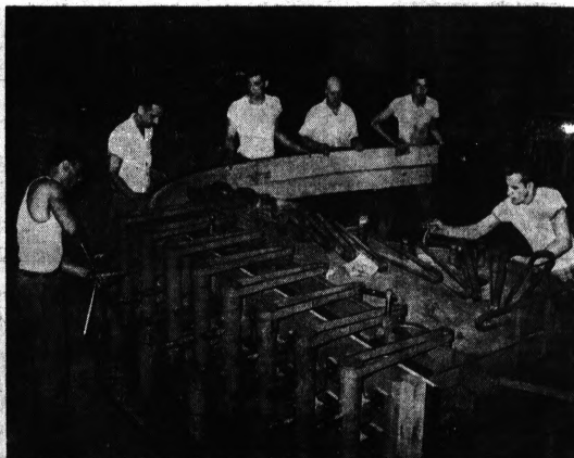
Using a steel press first devised 85 years ago, workmen bend the rim of a concert grand piano. As many as 22 layers of hard maple are glued together to assemble the rim.
