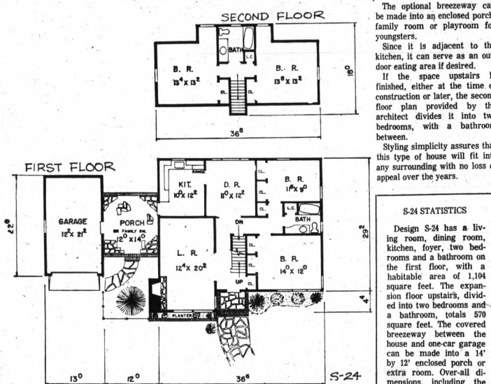
FLOOR PLANS: Architect has extra challenge in floor area of limited size, especially in the matter of privacy. Note here how two walls of closets act as sound barrier between the two bedrooms at the right side of house and the rest of the rooms.
