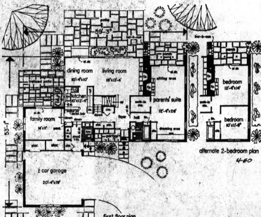
FLOOR PLANS — Whether you want a luxurious eight-room with a two-car garage, or an economical five-room cottage, or something in between, the plans for this house are flexible enough to permit fulfilling your family's needs.
