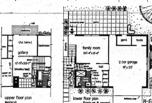
FLOOR PLANS: All the space advantages of a split level are present in this design, plus an eye-catching gallery that resembles a floating platform over the foyer.
