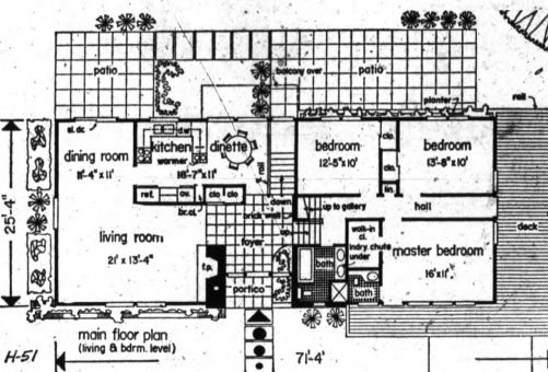
DISTINCTIVE SPLIT LEVEL: There are many unusual features in this split level house, among them an exterior wrap-around deck that can be entered from the master bedroom or the bedroom hall.
