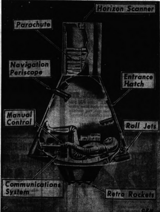
CAPSULE FOR MAN FLIGHT —This sketch, based on information supplied by the NASA, shows a cross-section of the Project Mercury ballistic capsule for America's first astronaut. It shows how the astronaut lies supine in the capsule and various controls and instruments in the space vehicle. Retro rockets at the bottom slow down the vehicle on its re-entry from space.
