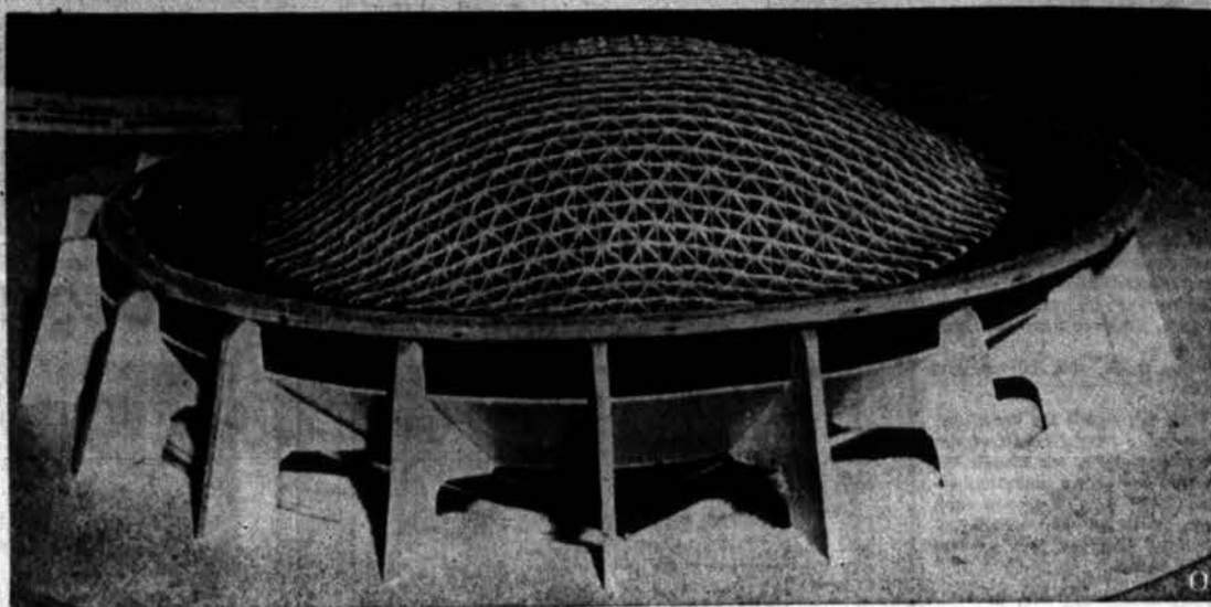
MODEL ARENA — Showing its dome, which would protect spectators from the weather, this model of the proposed Brooklyn Stadium demonstrates the new-as-tomorrow features which will be incorporated into the structure. It may be completed by 1958, and will seat 50,000 spectators. If it has the all-weather dome, the stadium will cost $9,000,000 and $7,000,000 if the roof is eliminated.
