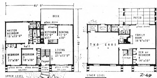
FLOOR PLANS — The six rooms on the upper level would be the livable area if this were the layout of a true ranch. Bilevel
