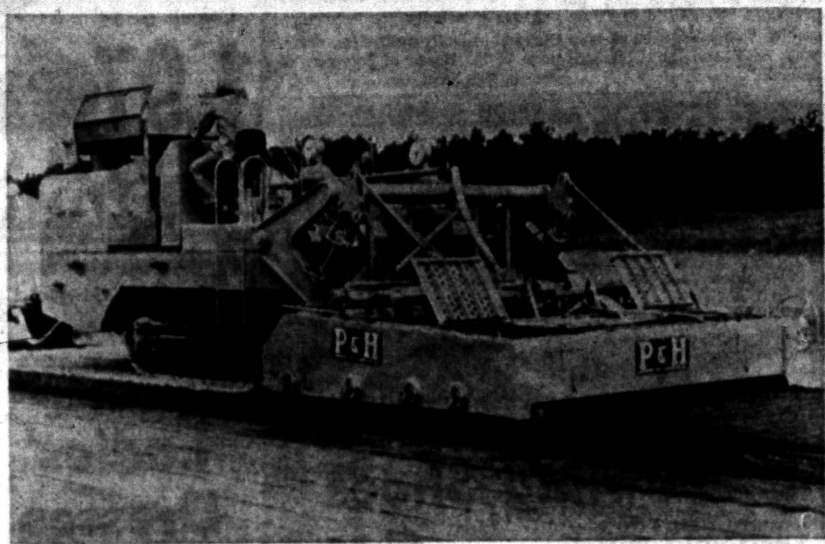
BUILDS RUNWAY — This is the soil cement machine which is being used to build the new, 4,000 foot east-west runway at Pontiac Municipal Airport. By mixing the topsoil, cement and water,
