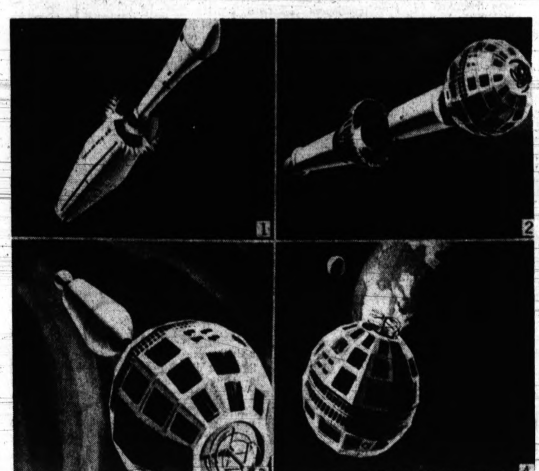
TELSTAR II — A three-stage Delta rocket launched the second U.S. communications satellite into orbit today, with every indication of success. First stage of the rocket separates (1), followed by second stage separation (2). Telstar II is released from the rocket's third stage (3) and moves into earth orbit (4).
