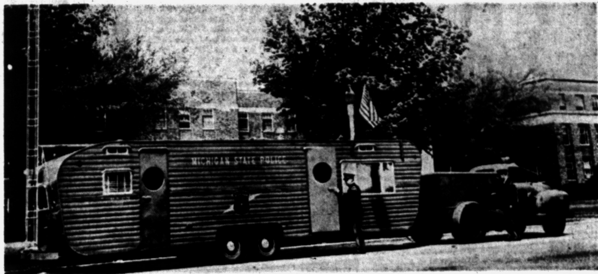
NEW STATE POLICE UNIT—Earmarked for use during disasters. The 33-foot house trailer is fitted out with radio transmitters, telephones, public address system and auxiliary power unit.
