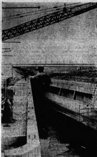
$44-MILLION ANSWER — When the 12-Towns Storm Relief Drain is completed in South Oakland County by early 1964, this concrete barrage, known as a weir, will divert sewage into the Detroit system for treatment, and funnel storm waters down the Red Run Drain into Lake St. Clair. More pictures and story on Page 15.
