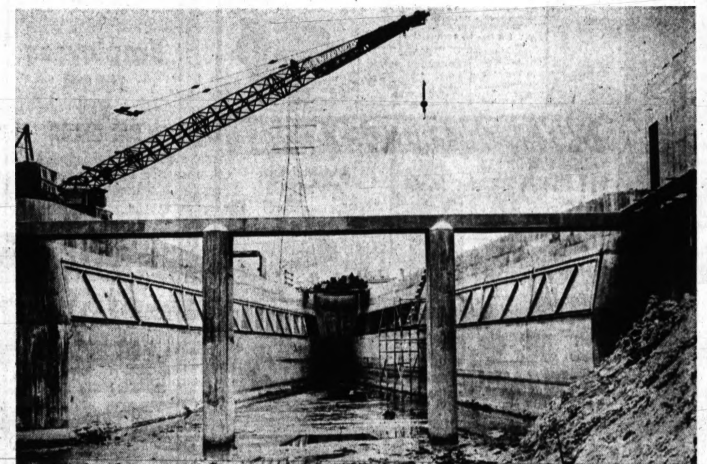
YAWNING JAWS — Known as a weir, this giant concrete maw will store storm waters and sewage long enough for the wastes to rise to the top, thence through aluminum chutes on either side into the Detroit sewage system. Remaining rain waters will flow through opened sluice gates at the far end into the Red Run drain and on to Lake St. Clair.
