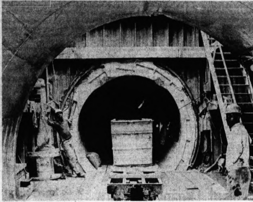
"HERE SHE COMES" — Workers stand back as a train load of clay emerges from the 9½-foot-high concrete tunnel. The clay was drilled out at the other end by a $100,000 mining machine that cuts through the earth at a rate of 50 feet per day.
